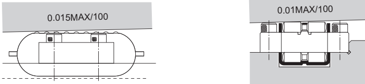
(a) Parallelism between the LM Roller and the raceway (b) Allowable tilt of the roller in the longitudinal direction
