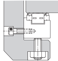
(b) Using a set screw
